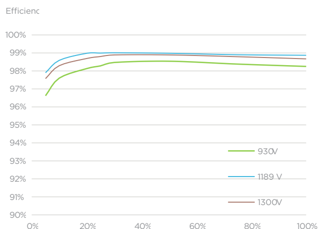
Efficiency Curve
